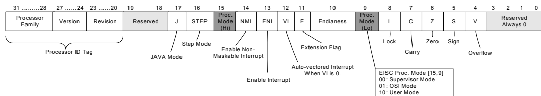
Figure 2.2: Status Register
