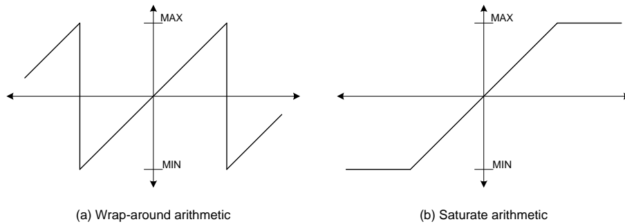
Figure 3.3: Saturate Arithmetic
