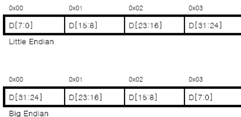
Figure 2.6: Endianness
